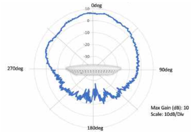
5 GHz Elevation
